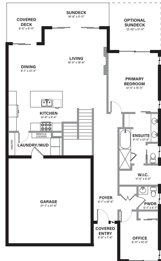
MAIN LEVEL
