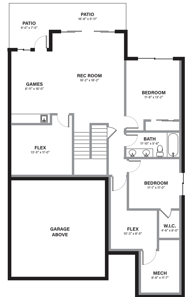
WALK-OUT LEVEL
