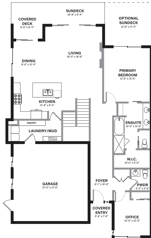
MAIN LEVEL
