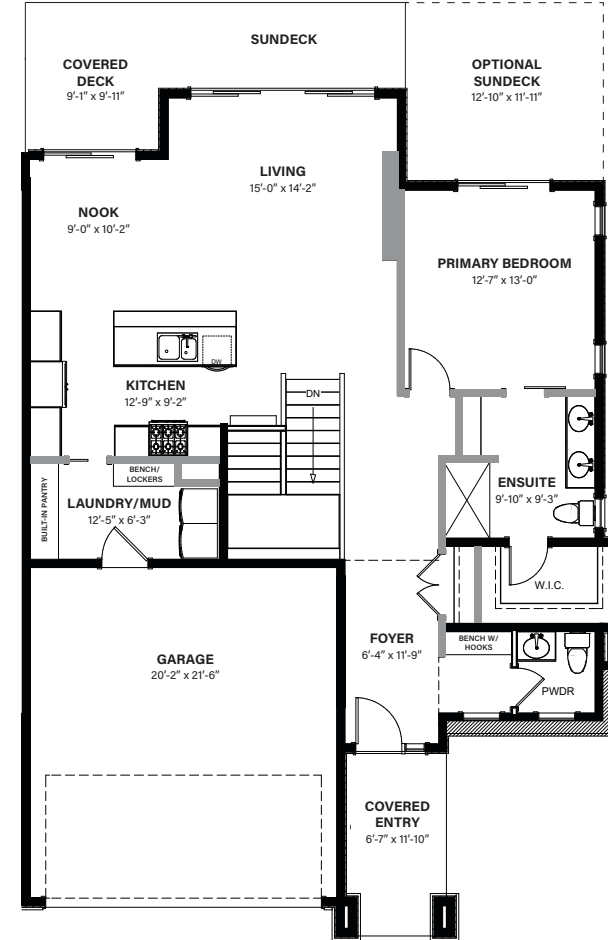
MAIN LEVEL
